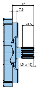
SHAFT CODE 4 SAE BB INVOLUTE SPLINE DATA CLASS 1 - FLAT ROOT SIDE FIT 4498b - PITCH 16/32 15 TEETH - 30° PRESSURE ANGLE
