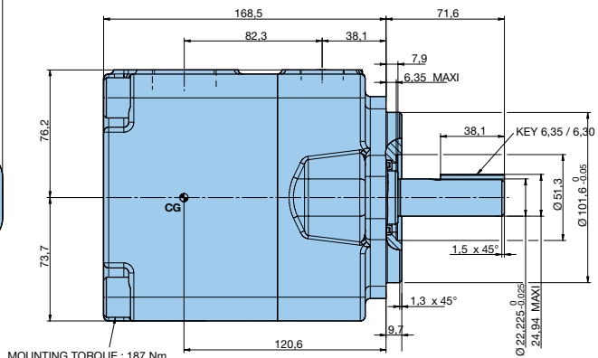
SHAFT CODE 1 (KEYED SAE B)
